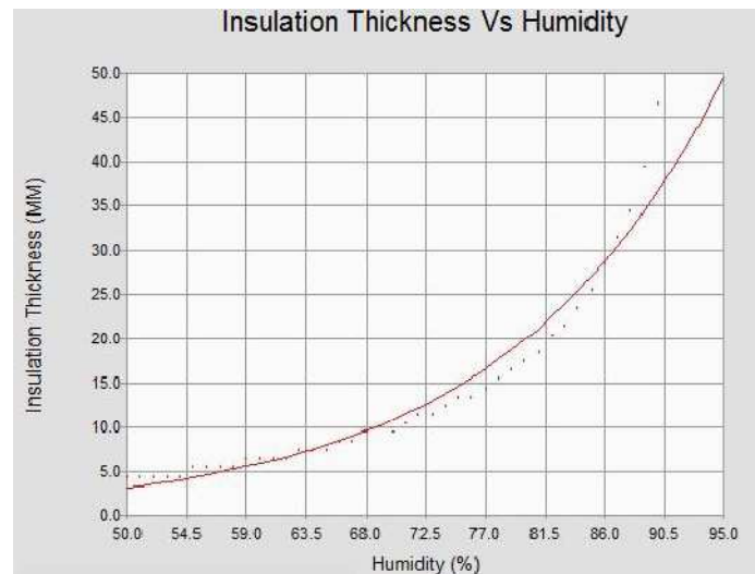
Figure 2: Thickness and humidity comparison example of a typical environment with ambient temperature of 30 °C and line temperature of 10 °C
