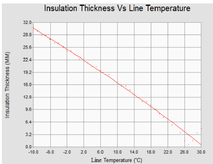
Figure 3: Thickness and line temperature comparison example of a typical environment with ambient temperature of 30 °C and humidity of 80%
